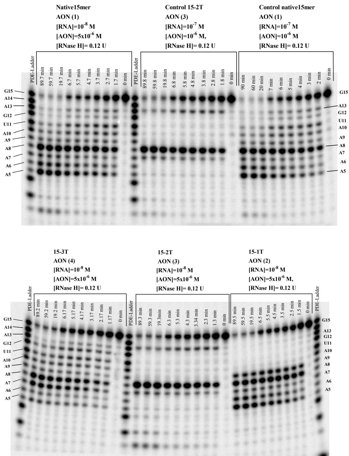
Figure S9. Autoradiograms of 20% denaturing PAGE, showing the cleavage kinetics of 5'- ^{32} P-labelled target RNA ( 14 ) by RNase H1 in the native AON ( 1 )/RNA ( 14 ) and single, double and triple oxetane T modified AON ( 2-4 )/RNA ( 14 ) hybrid duplexes. The kinetics of the control native 15mer AON ( 1 ) and double T AON ( 3 ) with 1 \mu M and RNA ( 14 ) with 0.1 \mu M concentration, used for the calibration of the exact RNase H concentration, are also shown. PDE-Ladder: snake venom PDE ladder. Conditions of cleavage reaction: RNA (0.01 or 0.1 \mu M) and AONs (1 or 5 \mu M) in buffer, containing 20 mM Tris-HCl (pH 8.0), 20 mM KCl, 10 mM MgCl 2 and 0.1 mM DTT at 21 °C, 0.12 U of RNase H. Total reaction volume is 30 \mu l. (See Materials and Methods section for full experimental details.)
